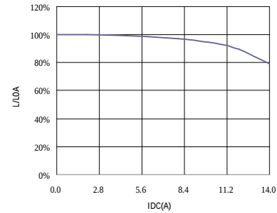
SR0805100ML□
