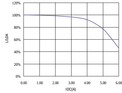
SR0805820KL□
